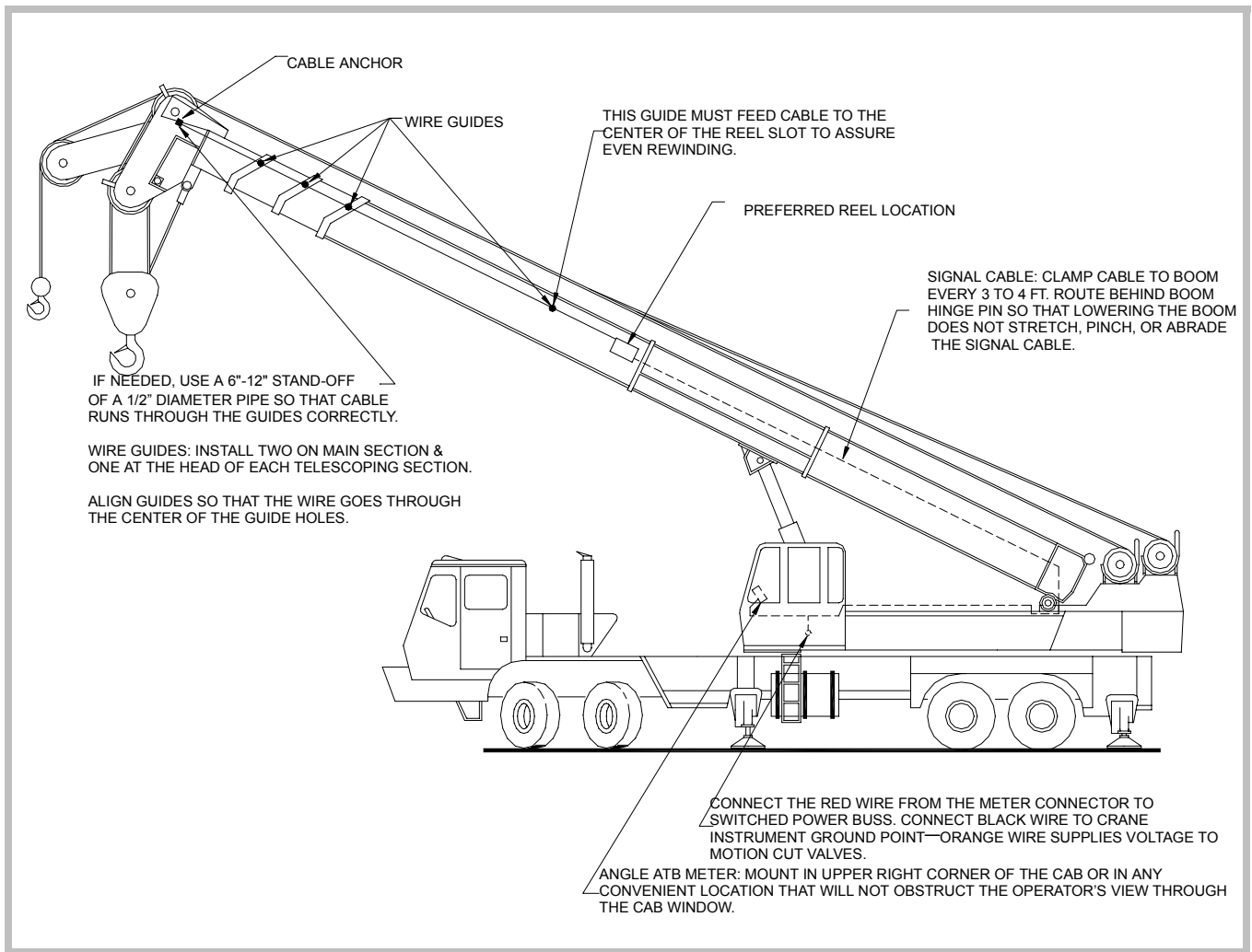
FIGURE 1: THE BB™ 508/509 ANTI TWO-BLOCK ALARM SYSTEM SET UP ON A HYDRAULIC CRANE
