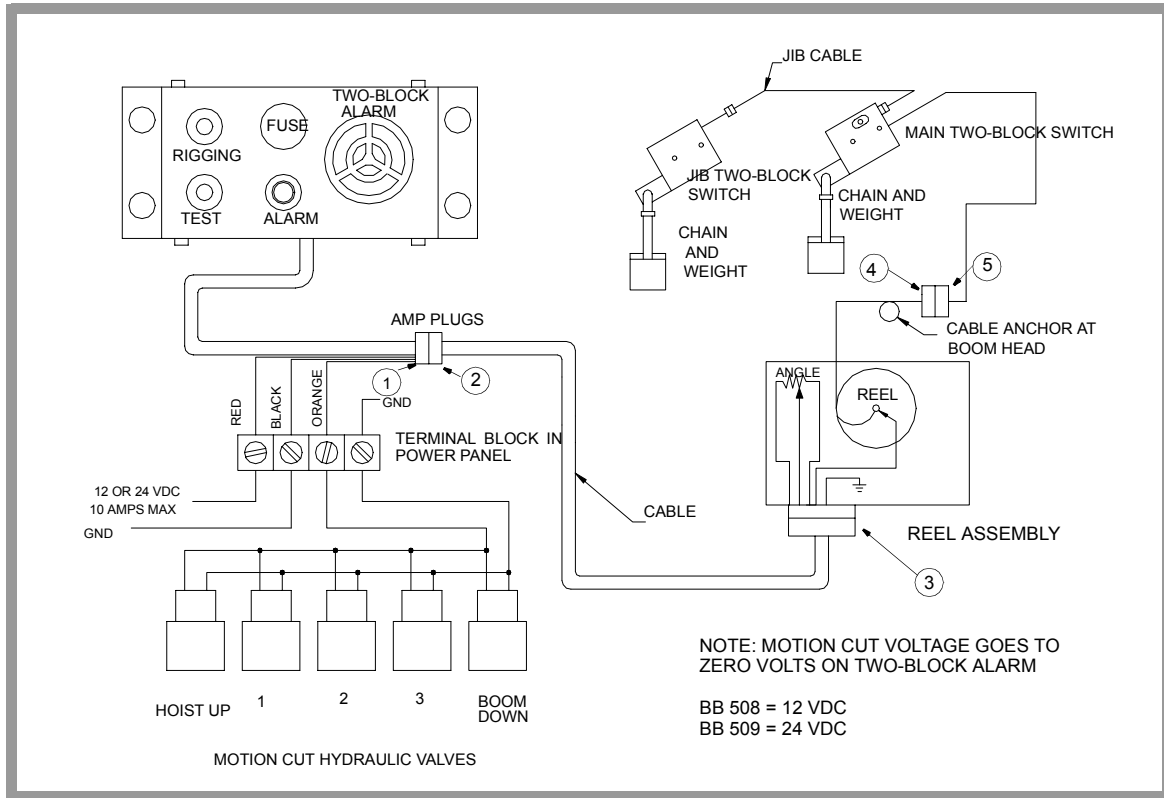
FIGURE 2: THE BB™ 508/509 SYSTEM LAYOUT
